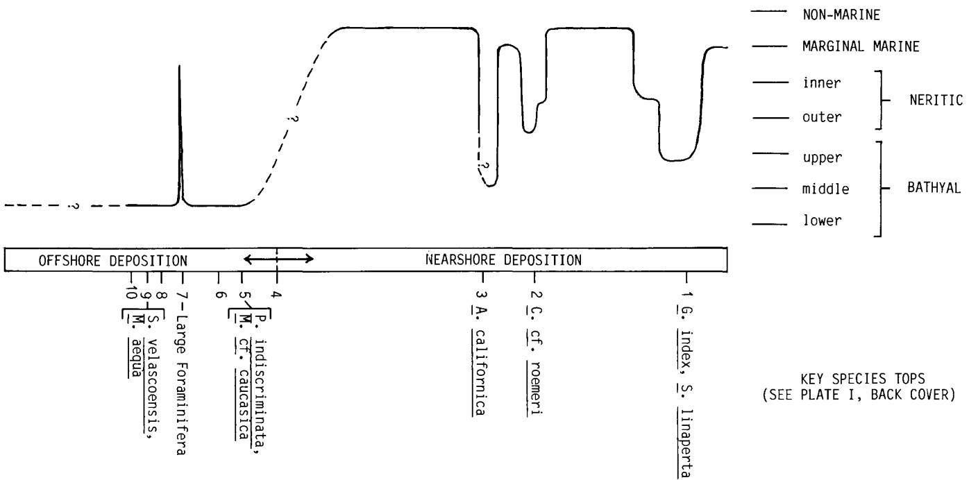
Figure 1. Generalized biostratigraphy and paleobathymetric curve for composited well section, southwest Oregon. Paleogene planktic zones after Blow (1979).
